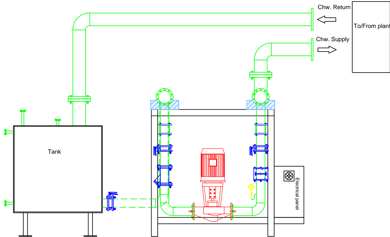
TRADITIONAL PUMP SKID
