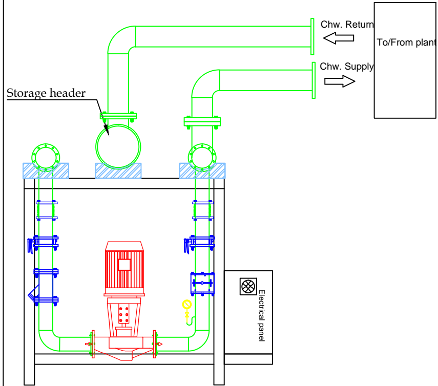
PROPOSED PUMP SKID
